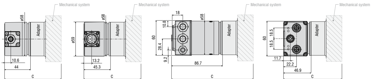
HTL/TTL output
