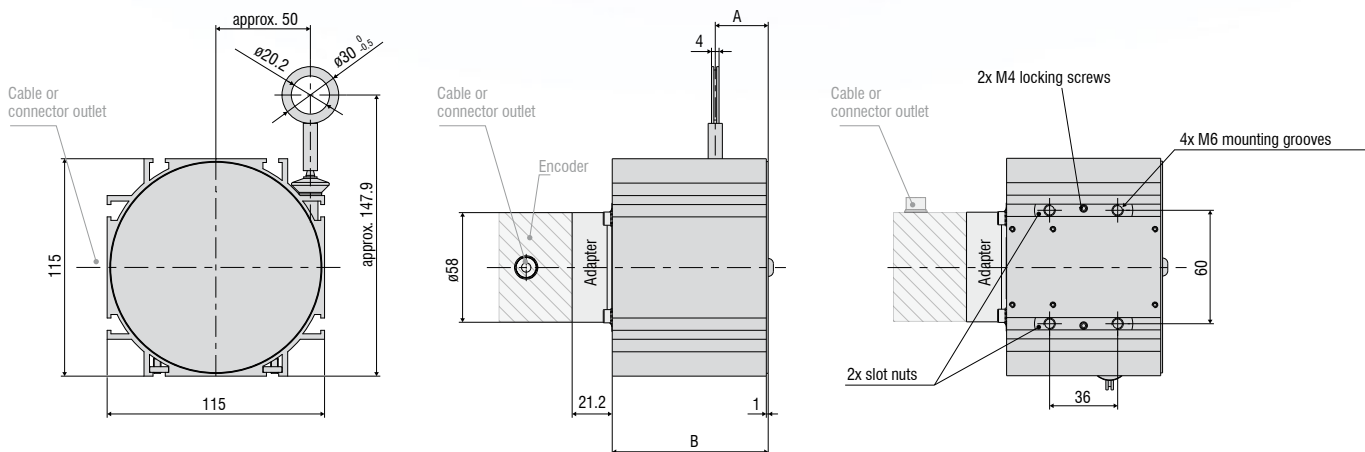
HTL/TTL output
